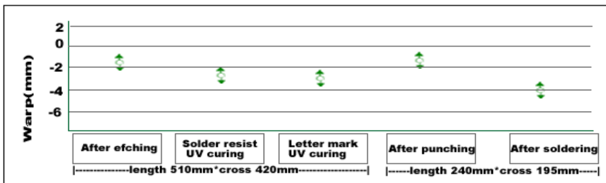
Warping through PCB process (thickness 1.6mm single side)
