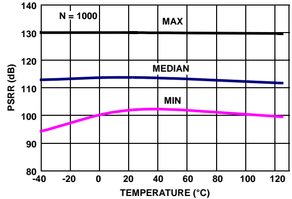
FIGURE 48. ISL28276, ISL28476 PSRR vs TEMPERATURE, V_+, V_- = \pm 1.2V TO \pm 2.5V
