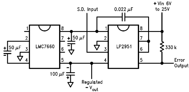
FIGURE 12. Regulated -5V with 200 µA Standby Current
